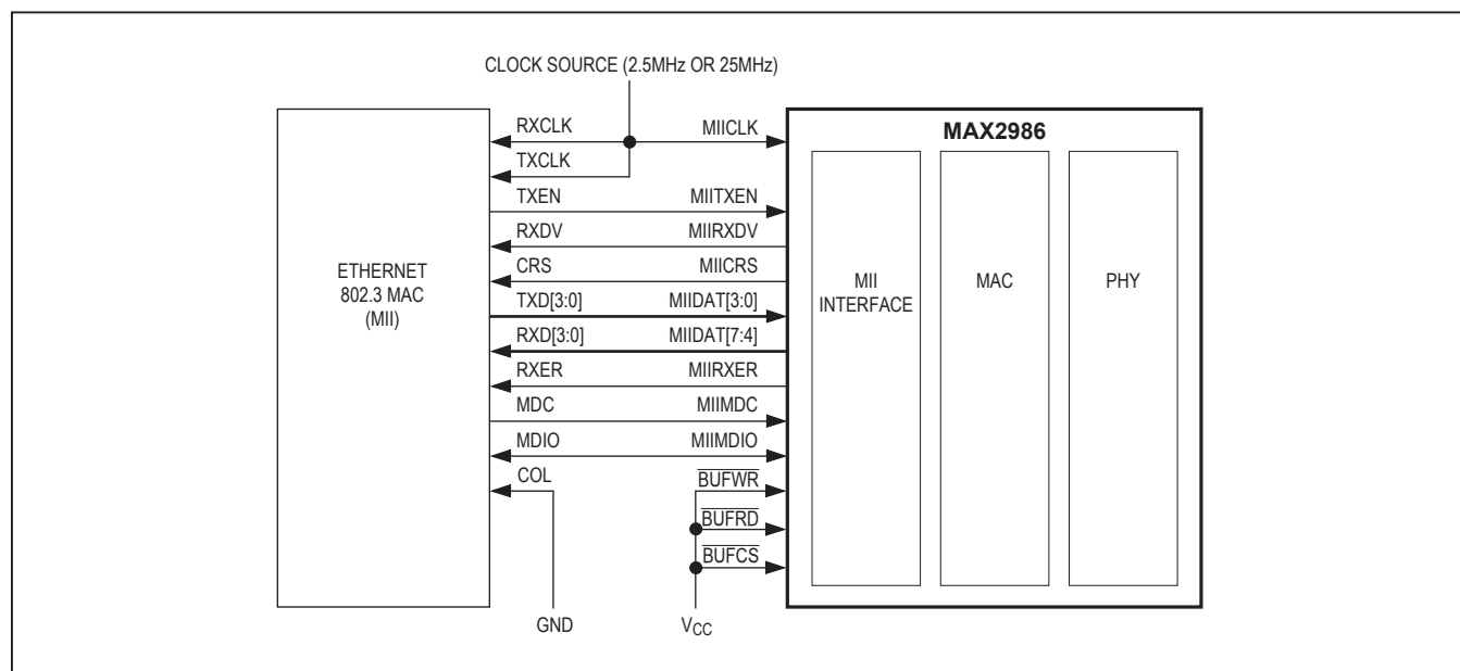
Figure 3. MAC and PHY Connection in MII Mode
